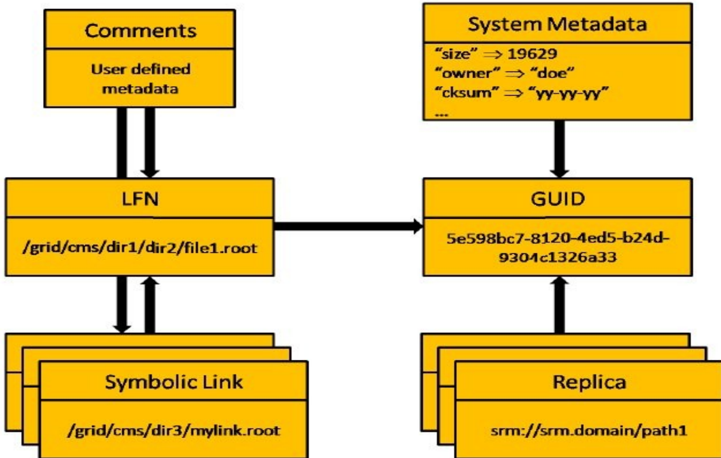
LFC architecture
